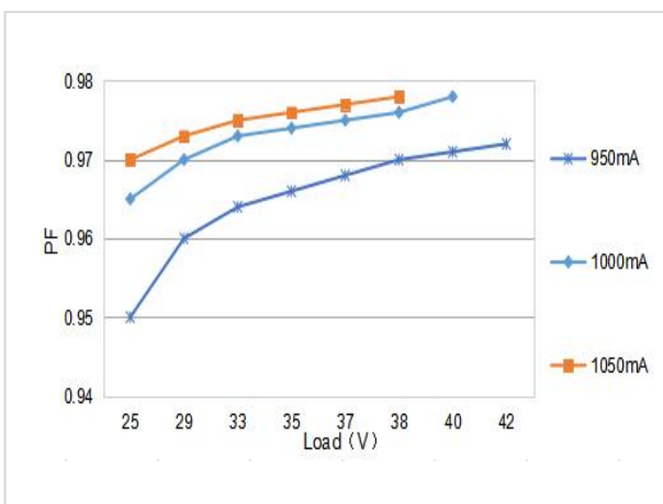
PF Curve 2
