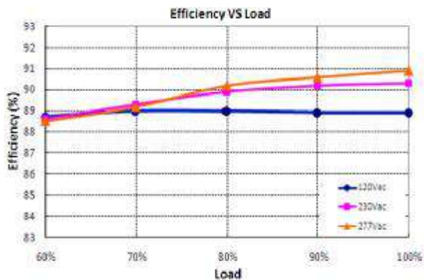
X6-075Y108 (Io=0.7A)
