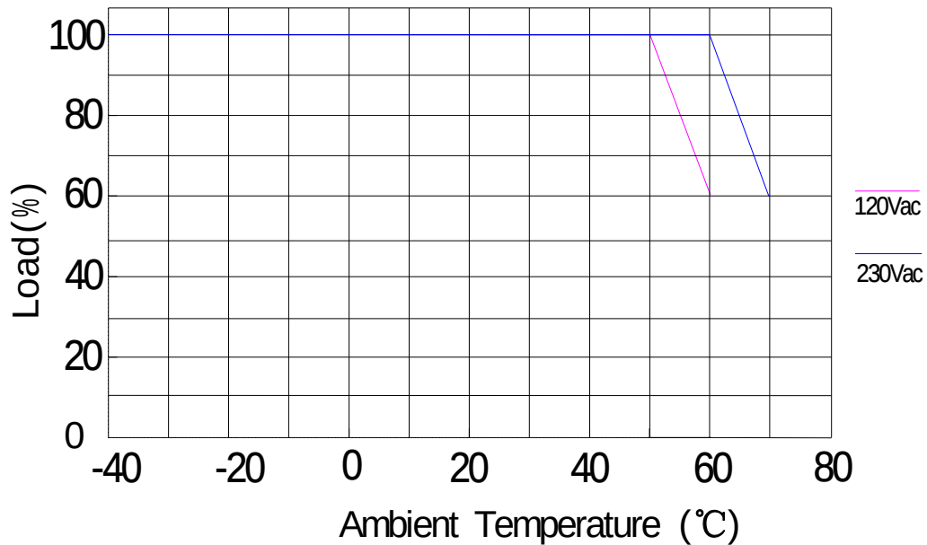
Derating Curve
