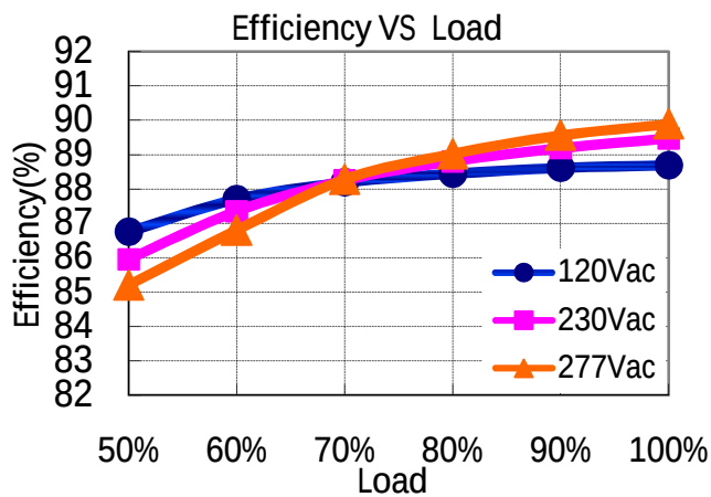
X6-075Y108 (Io=0.7A)
